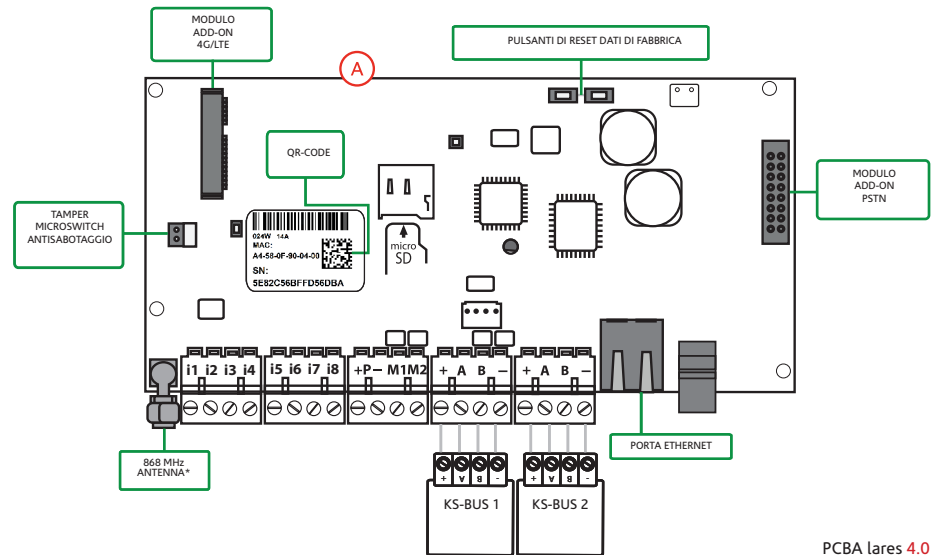
PCBA lares 4.0
